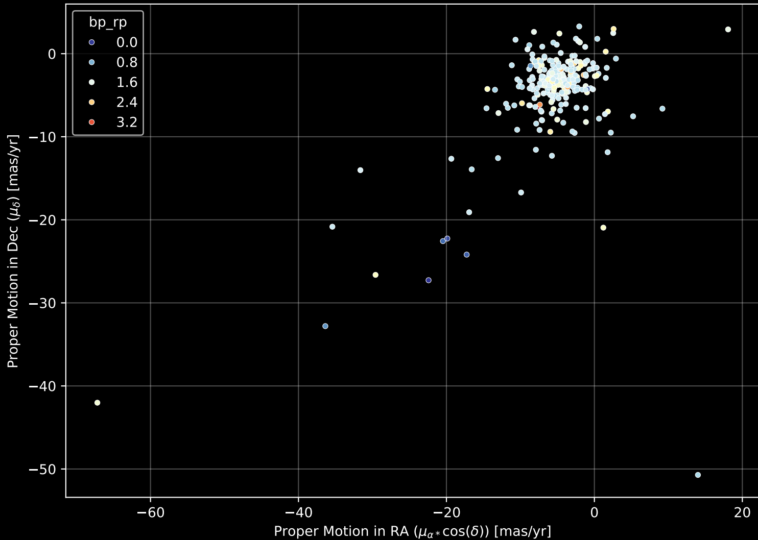
APOGEE DR17 Field: [330+12] Proper Motion Diagram (n= 248)
