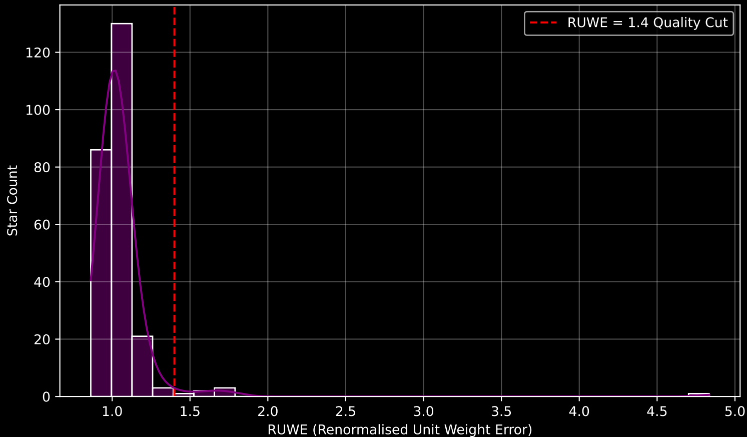
GAPOGEE DR17 Field [330+12] RUWE Distribution (n= 247)
