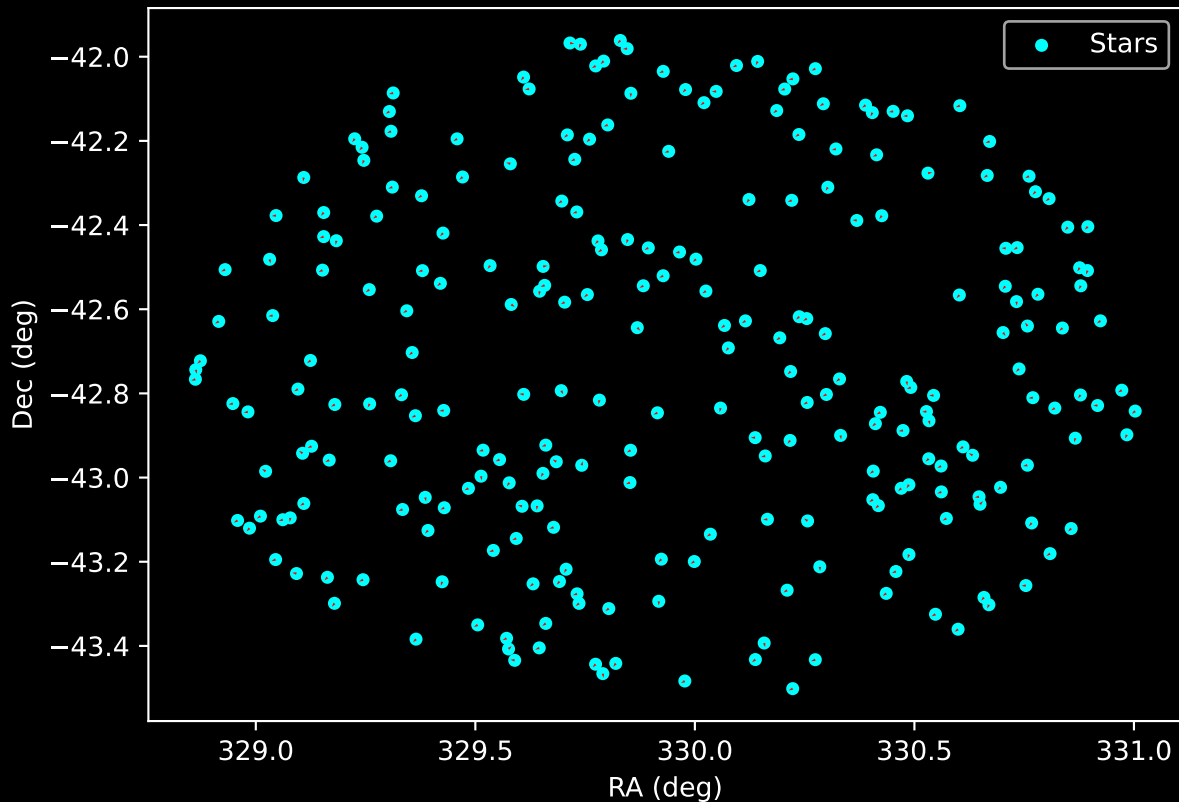
APOGEE DR17 Field: [330+12] Proper Motion Vectors for Gaia Star Field (n= 248)
