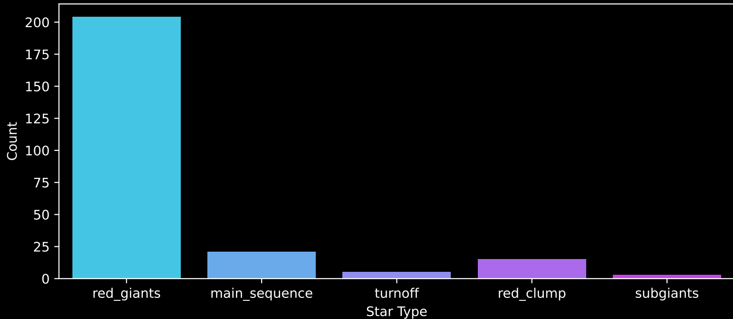
APOGEE DR17 Field: [330+12] Count plot of Star Type
