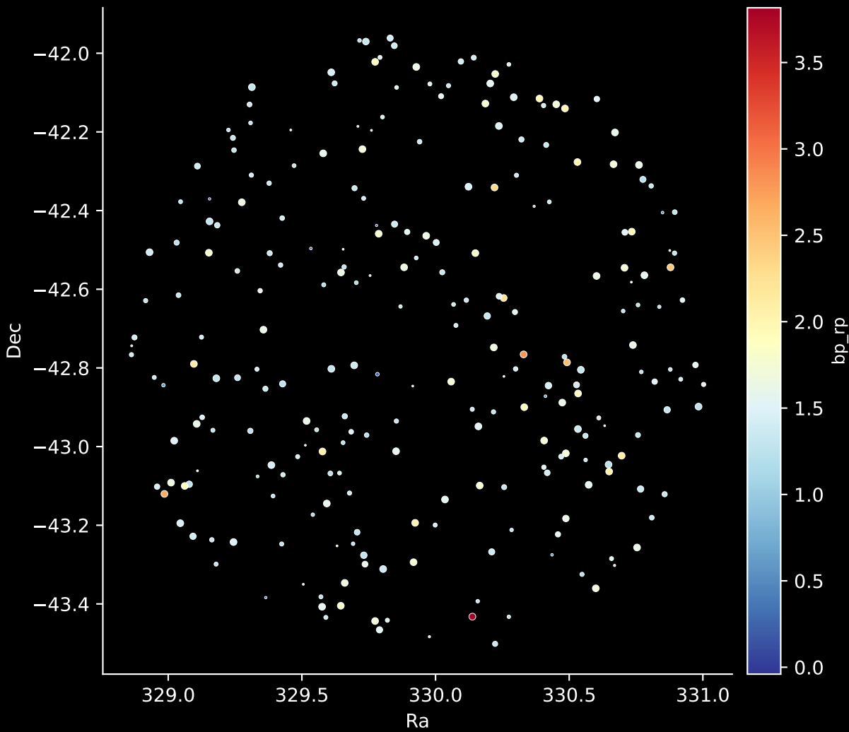
APOGEE DR17 Field: [330+12] Stars: 248
