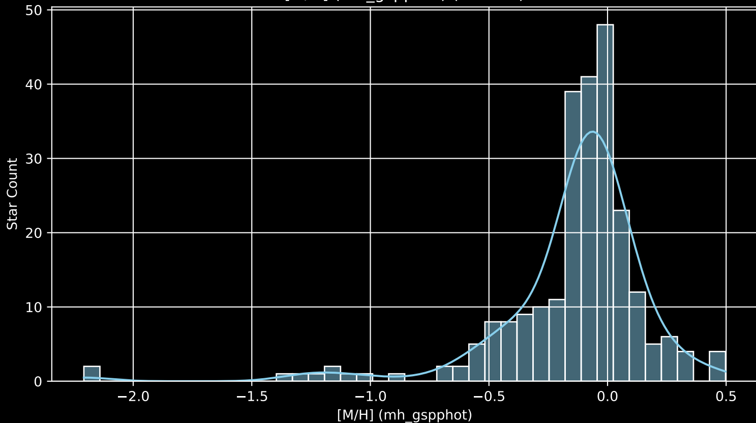
APOGEE DR17 Field: [330+12 [M/H] (mh_gspphot) (n= 247)
