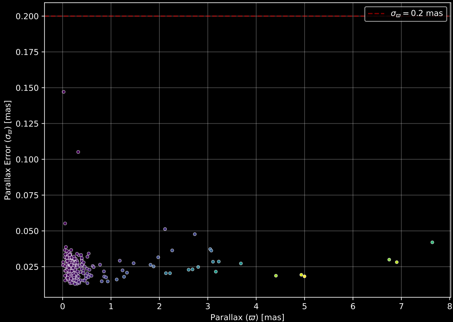
APOGEE DR17 Field: [330+12] Parallax Quality (n= 248)
