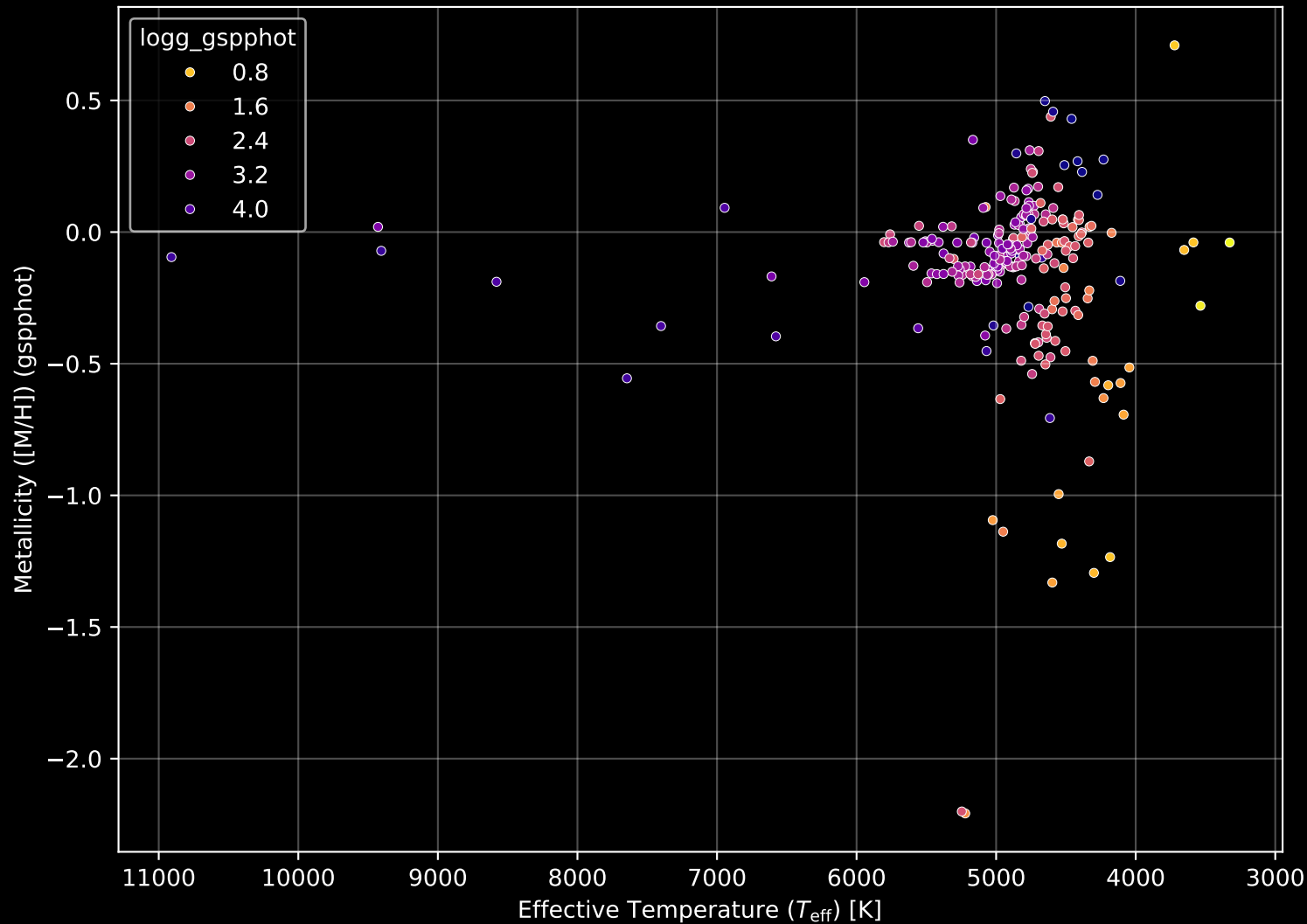
APOGEE DR17 Field: [330+12] Stellar Population Parameters (n= 248)
